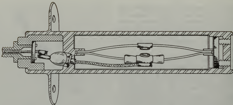
FIGURE 9-5. Fenwal spot detector.
